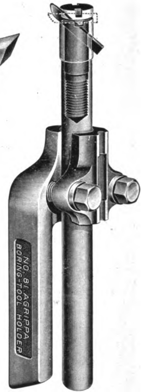
The Boring Tool takes any size or shape of bar and requires no bushings. Its sleeve bar cap admits a straight or angular cutter; either can be quickly inserted at the business end of the bar without removing the cap or disturbing the setting of either the bar or the holder.
